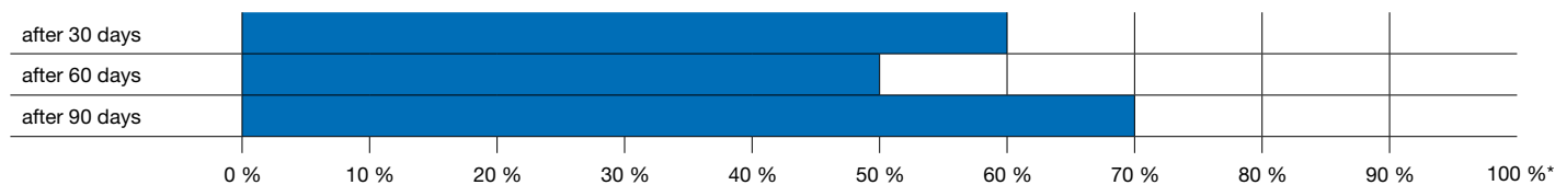
Tensile shear strength in % after storage in tropical climate in accordance with DIN 50015 (+40°C/+140°F and 92% humidity)
